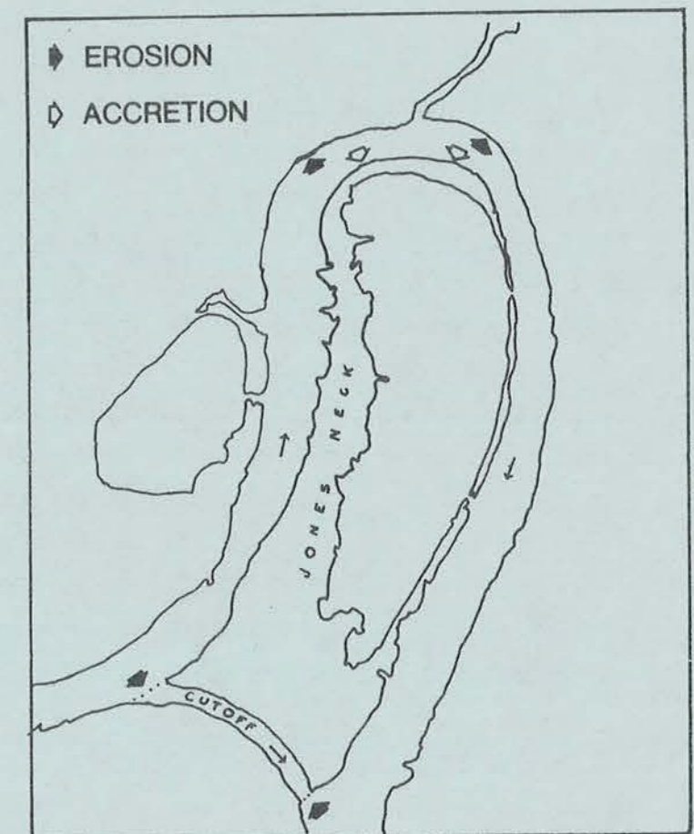
FIGURE 3. TYPICAL RIVER MEANDER
